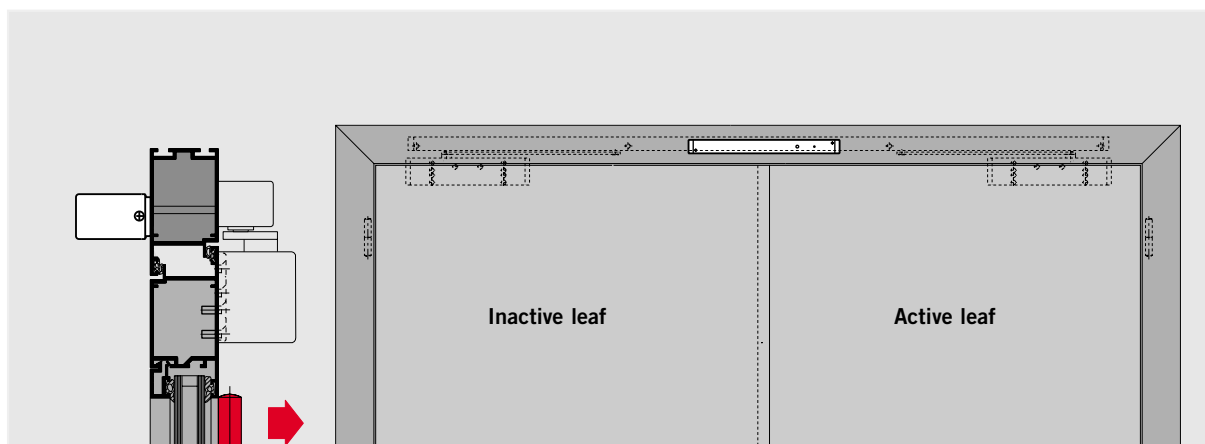
RMZ-K/S frame-mounted smoke detector on the push side connected to a G 93 GSR on the pull side
