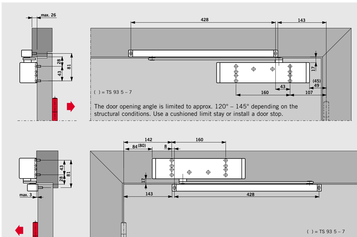
DORMA TS 93 G door closer with DORMA G 93 N slide channel assembly, door leaf fixing on the push side and transom fixing on the pull side. Examples: Anticlockwise-closing (ISO 6) door; mirrored arrangements apply to clockwise-closing (ISO 5) doors.
