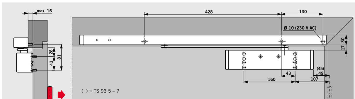
DORMA TS 93 G door closer with DORMA G 93 EMR slide channel assembly, push-side fixing Example: Anticlockwise-closing (ISO 6) door; mirrored arrangements apply to clockwise-closing (ISO 5) doors.
