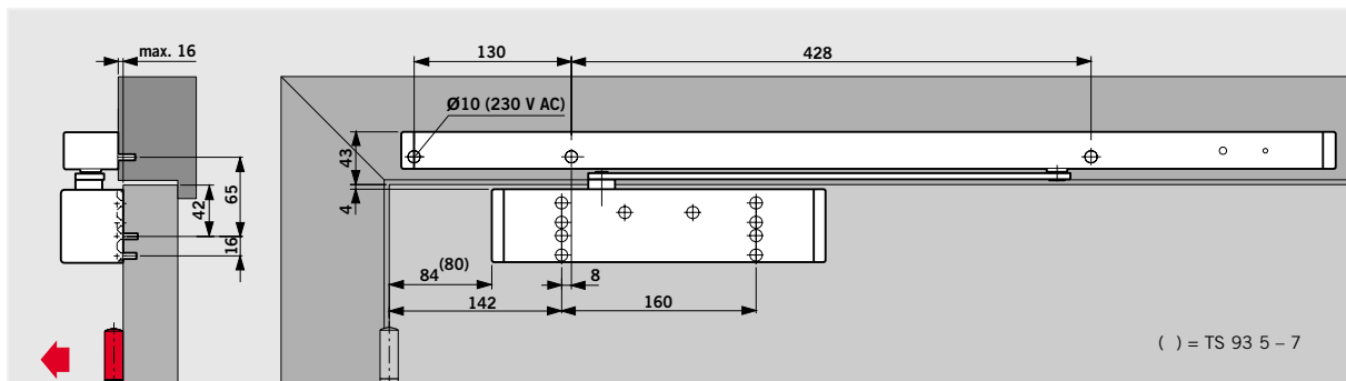
DORMA TS 93 B closer with DORMA G 93 EMR slide channel assembly, pull-side fixing Example: Anticlockwise-closing (ISO 6) door; mirrored arrangements apply to clockwise-closing (ISO 5) doors.
