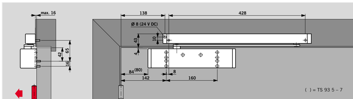
DORMA TS 93 B closer with DORMA G 93 EMF slide channel assembly, pull-side fixing Example: Anticlockwise-closing (ISO 6) door; mirrored arrangements apply to clockwise-closing (ISO 5) doors.
