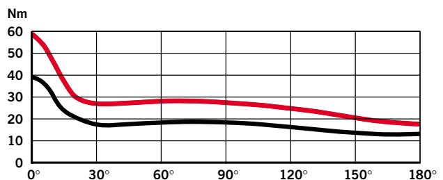
Force profile DORMA TS 93 (Spring strength: EN 5) — Opening force — Closing force
