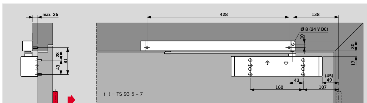
DORMA TS 93 G closer with DORMA G 93 EMF slide channel assembly, push-side fixing Example: Anticlockwise-closing (ISO 6) door; mirrored arrangements apply to clockwise-closing (ISO 5) doors.
