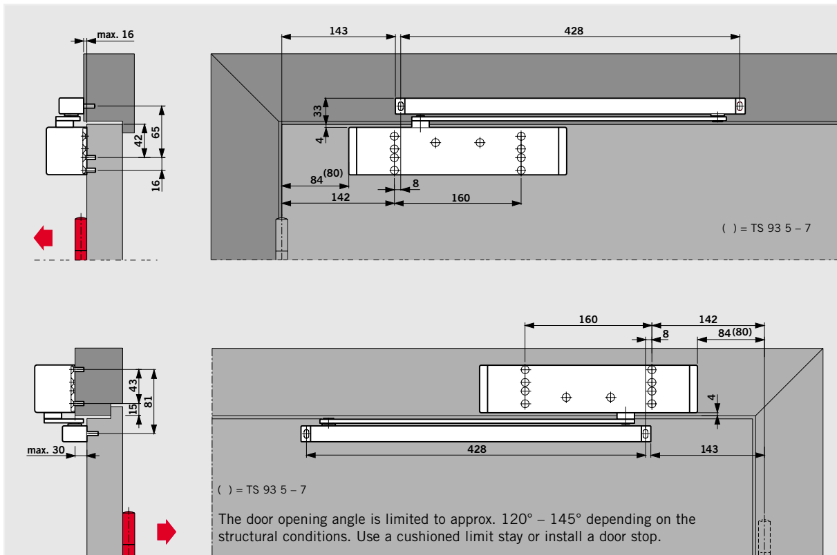
DORMA TS 93 B door closer with DORMA G 93 N slide channel assembly, door leaf fixing on the pull side and transom fixing on the push side. Examples: Anticlockwise-closing (ISO 6) door; mirrored arrangements apply to clockwise-closing (ISO 5) doors.
