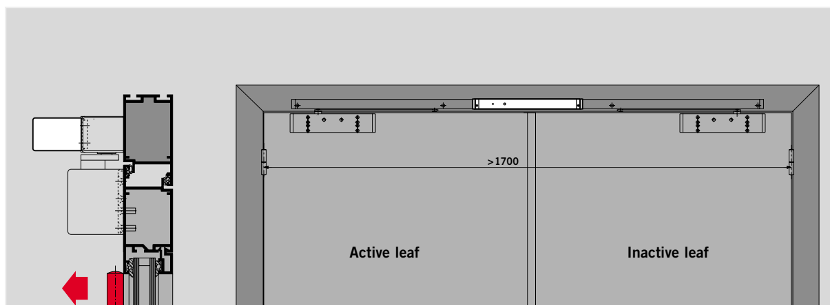
RMZ-K/S frame-mounted smoke detector on the pull side connected to a G 93 GSR on the pull side (use mounting bracket)
